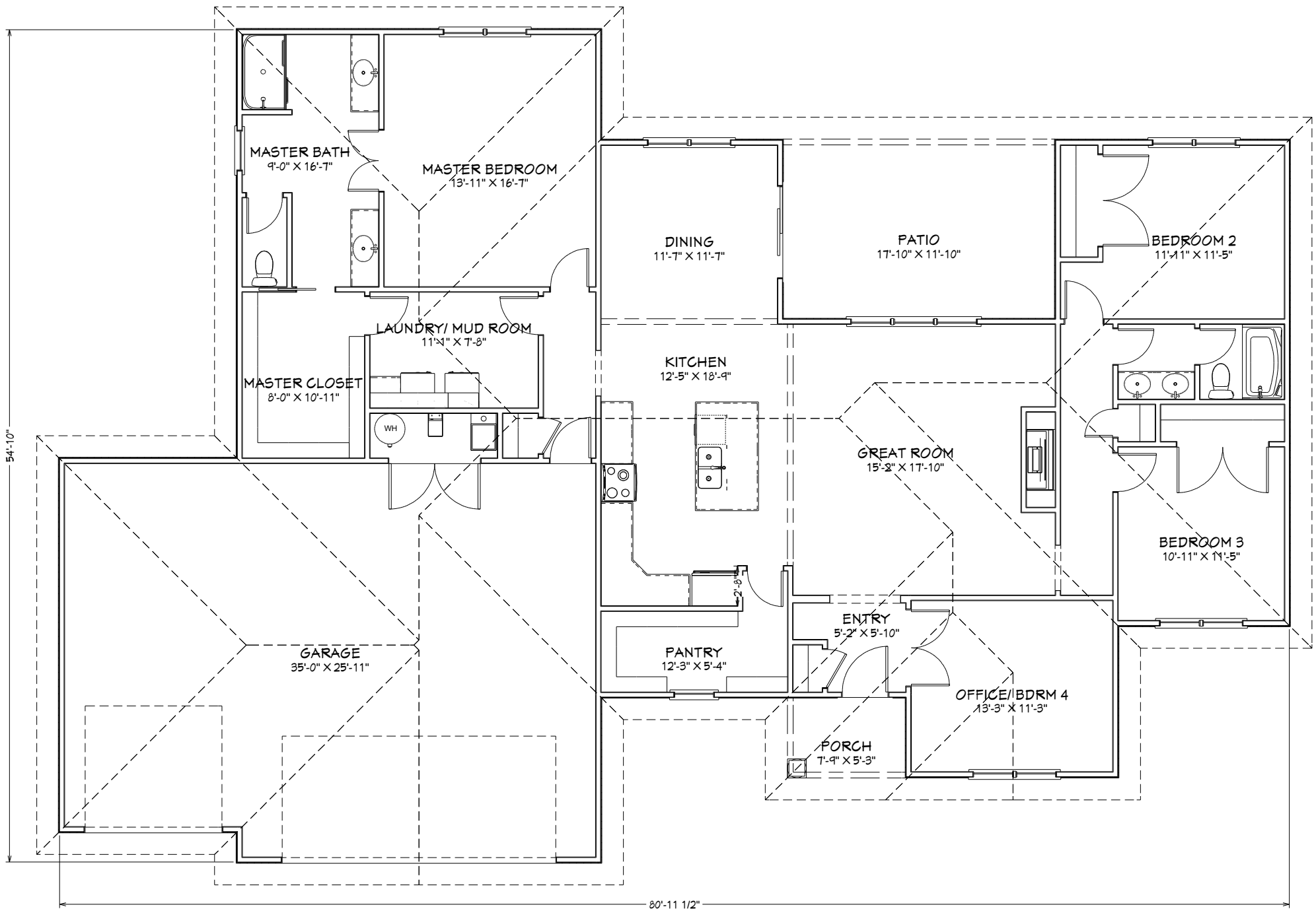
The Hickory LIVING AREA 2157 SQ FT
